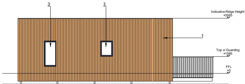
REAR ELEVATION
